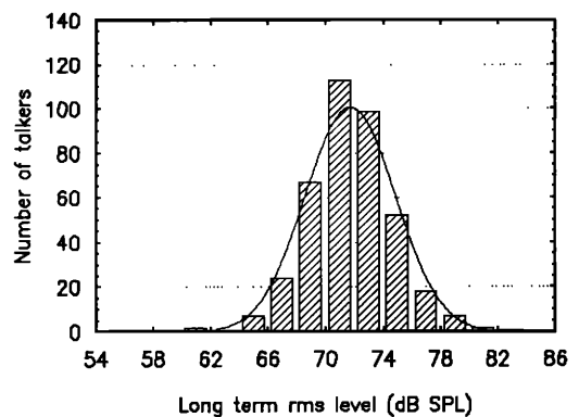
FIG. 5. Distribution of overall rms levels (measured at 20 cm from mouth). Curve shows normal distribution fitted to data.
